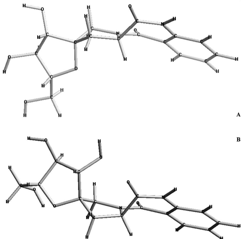
Figure 4. Oxygen-substituent pseudo-axial (A) and pseudo-equatorial (B) conformers of pyrrolo ring in compound 15 . Pseudo-axial conformer: total energy = 25.028 kcal/mol, dihedral angle C5a–C9a–N10–C11 = +16.91°; pseudo-equatorial conformer: total energy = 22.319 kcal/mol, dihedral angle C5a–C9a–N10–C11 = +17.32°.
